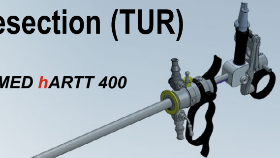
Bipolar Resectoscope
